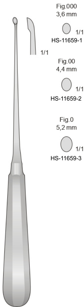
SIMON HS-11659 235 mm
