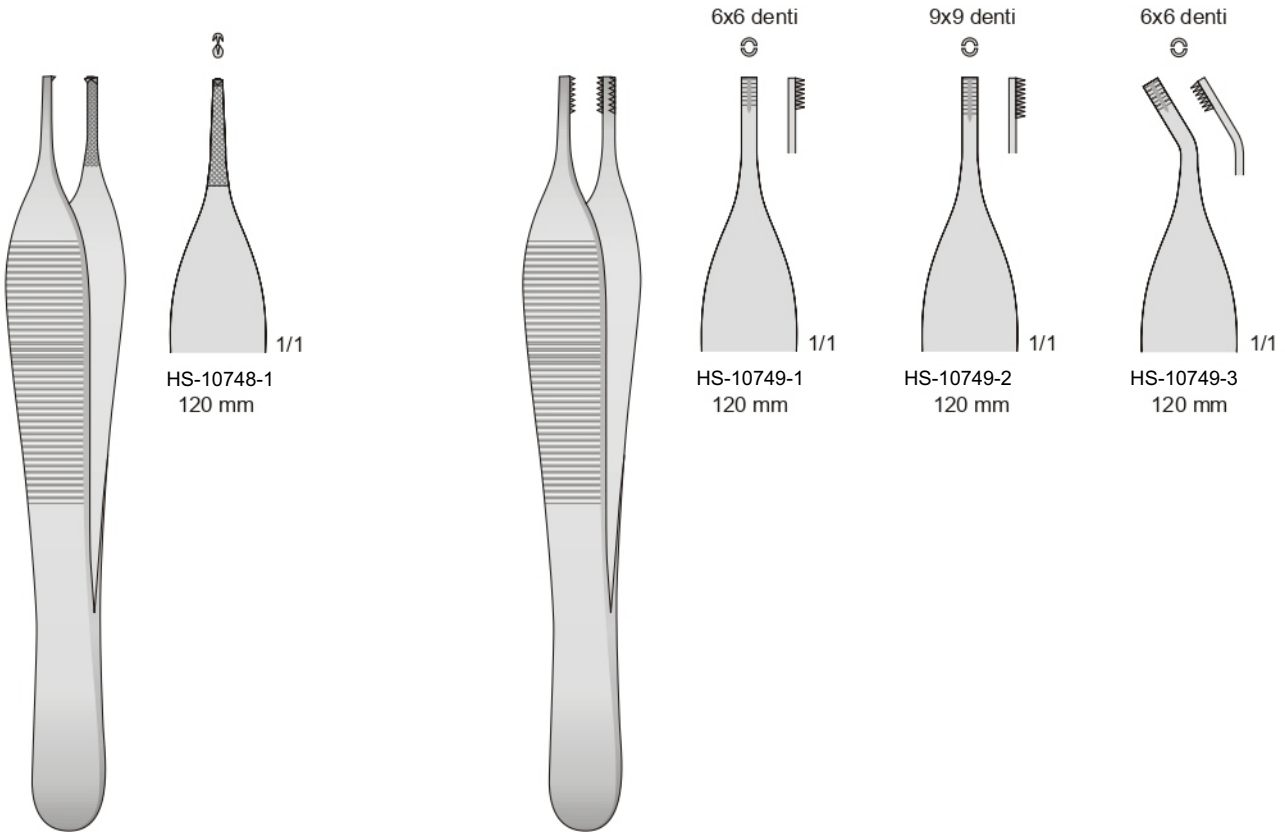
ADSON HS-10748 120 mm
