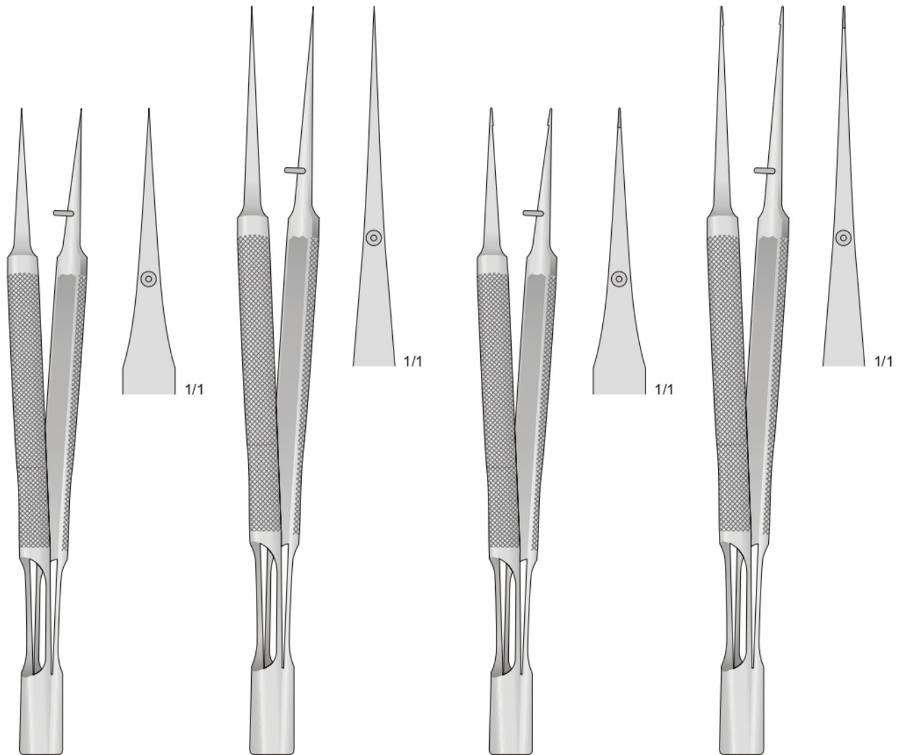
BROCK HS-10711 130 mm
