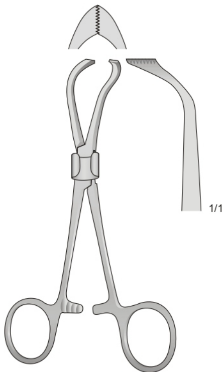
HS-7639-1 Ø 9 mm HS-7639-3 Ø 12 mm HS-7639-2 Ø 14 mm HS-7639-4 Ø 17 mm 100 mm
