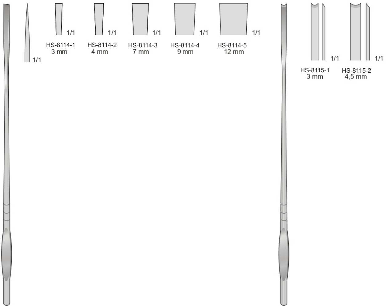
HS-8114 190 mm
