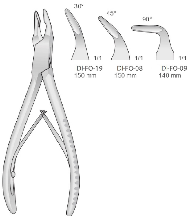
BLUMENTHAL DI-FO-08/ DI-FO-19
