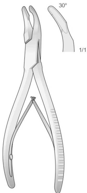
CLEVELAND DI-FO-231 140 mm DI-FO-232 170 mm
