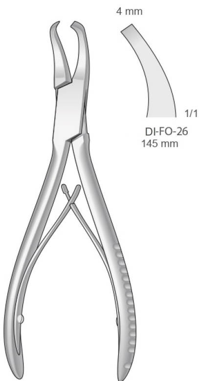
GARDNER DI-FO-26/ DI-FO-77 145 mm
