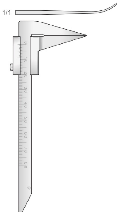
DI-DP-724 80 mm
